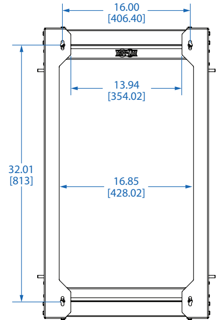
BACK VIEW
