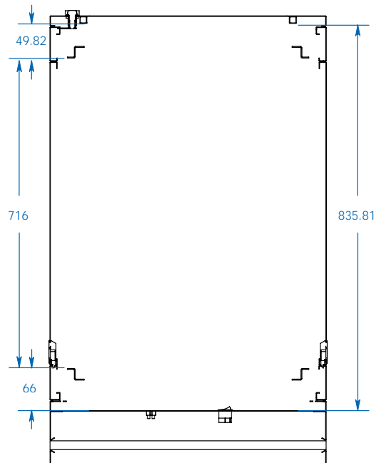
CROSS SECTION A USABLE MOUNTING DEPTH
