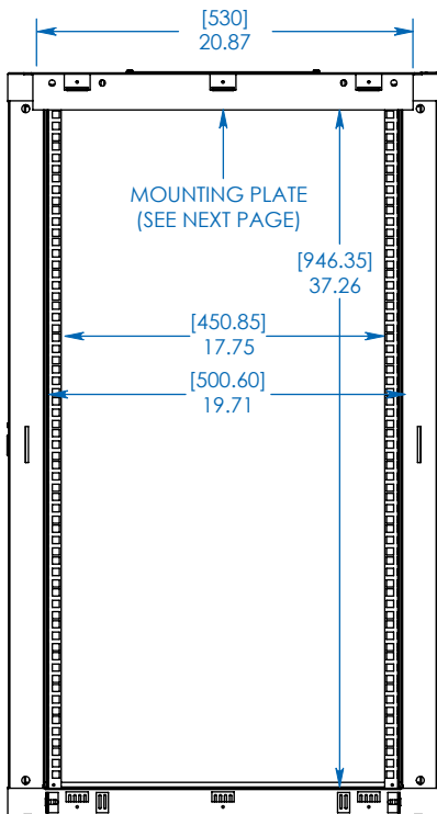
REAR VIEW (FRONT DOOR NOT SHOWN)
