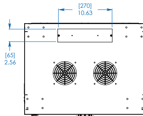
TOP/BOTTOM VIEW
