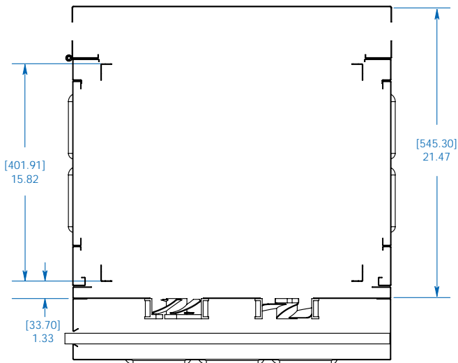
CROSS SECTION A USABLE MOUNTING DEPTH
