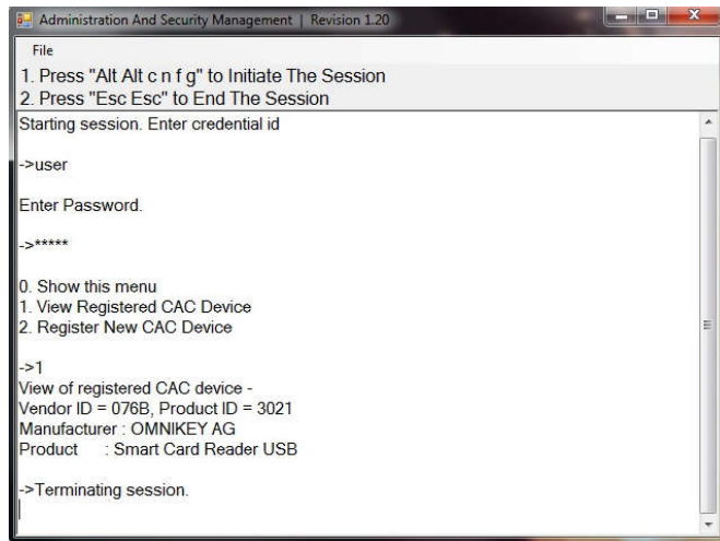
Figure 6: Terminate Session
