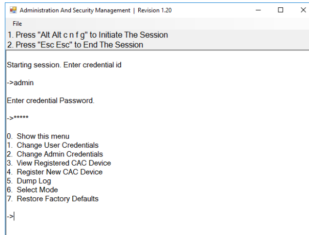
Figure 7: Administrator Log-in
