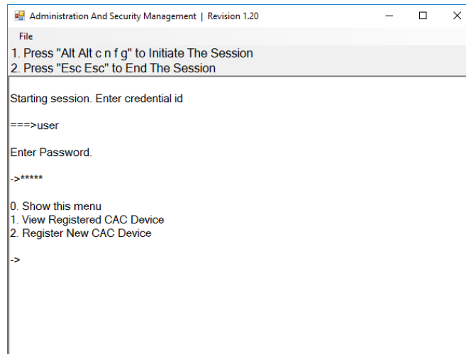
Figure 3: User Log-in
